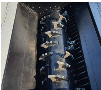
Shredding Unit
