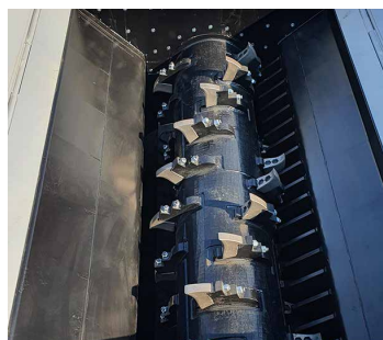
Shredding Unit
